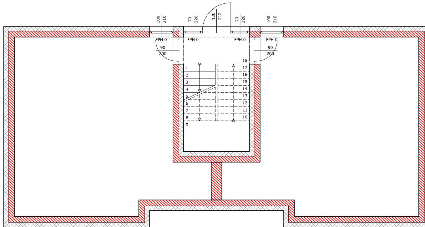
Grundriss M= 1: 100
