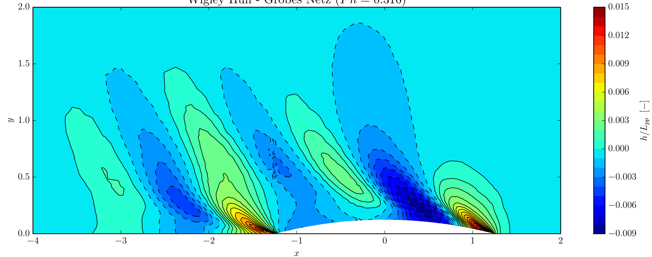
Wigley Hull - Grobes Netz ( Fn = 0.316 )
