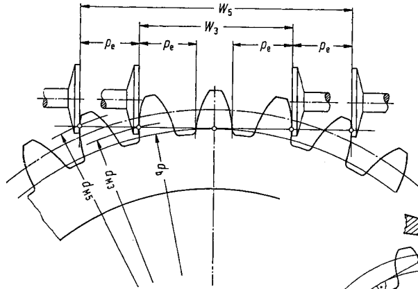
Measurement of Base tangent length
