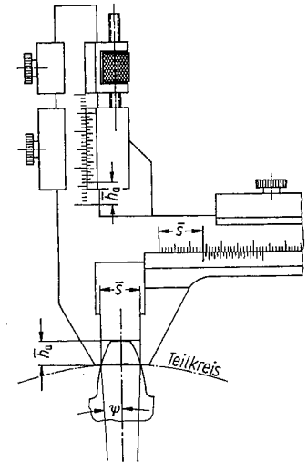
Measurement of tooth thickness
