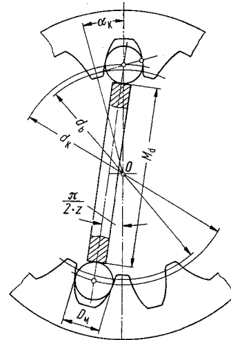
Measurement over rollers
