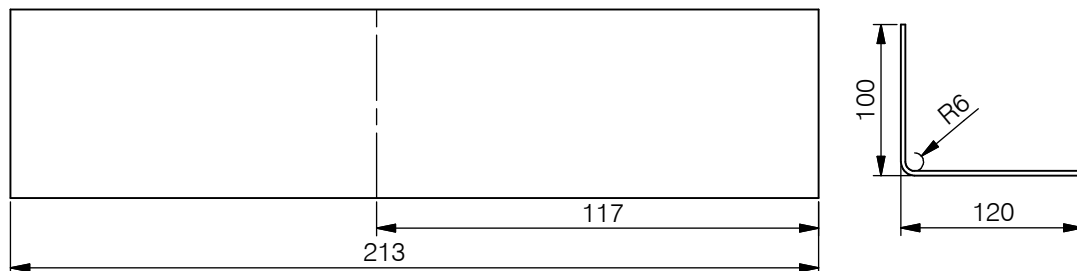
Winkel 120x100x3
