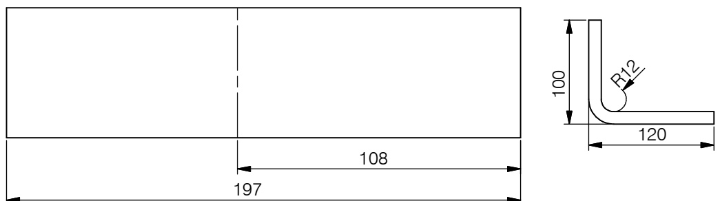
Winkel 120x100x12
