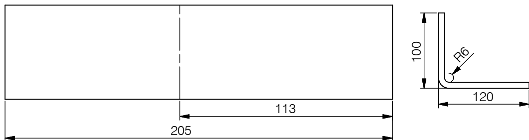
Winkel 120x100x8
