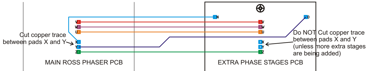
CONNECTION TO MAIN PCB
