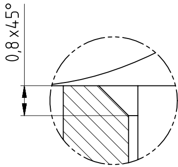
DETAIL Z SCALE 10:1
