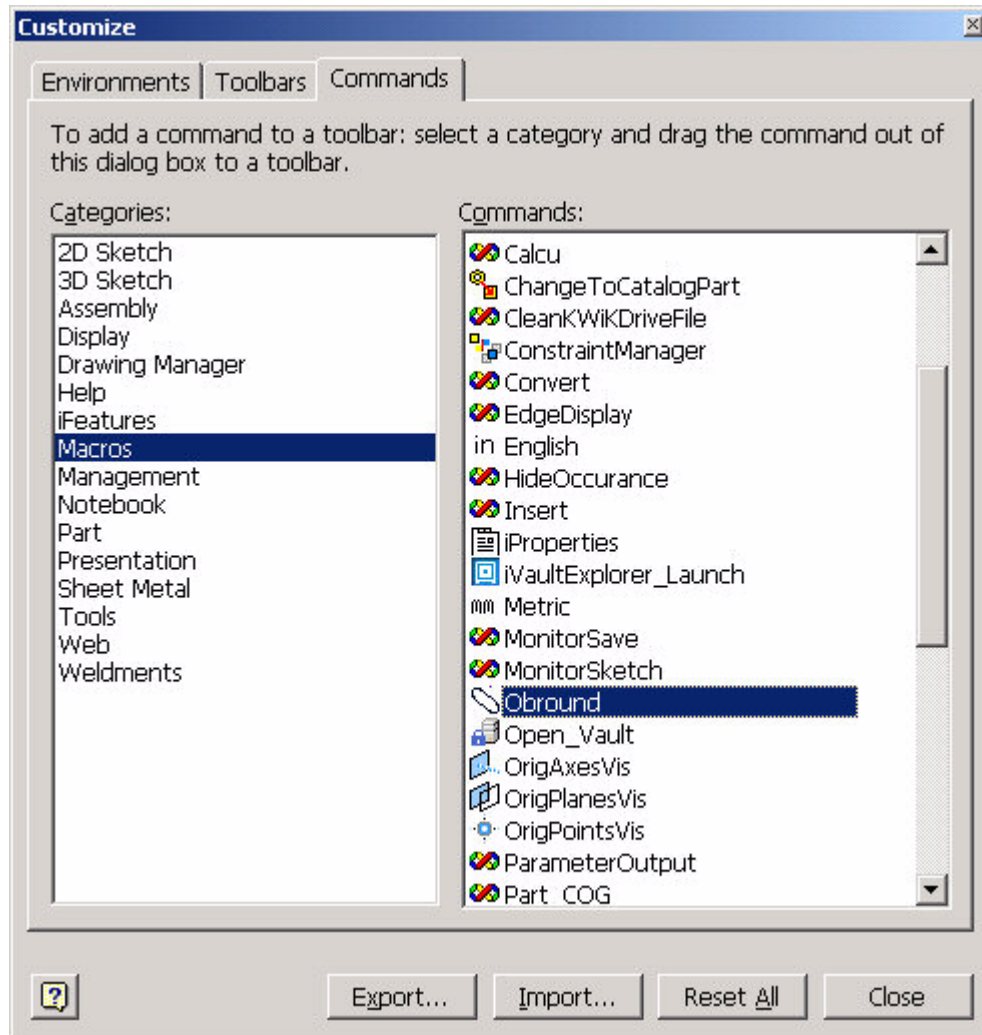
Figure 9 - Available Macros
