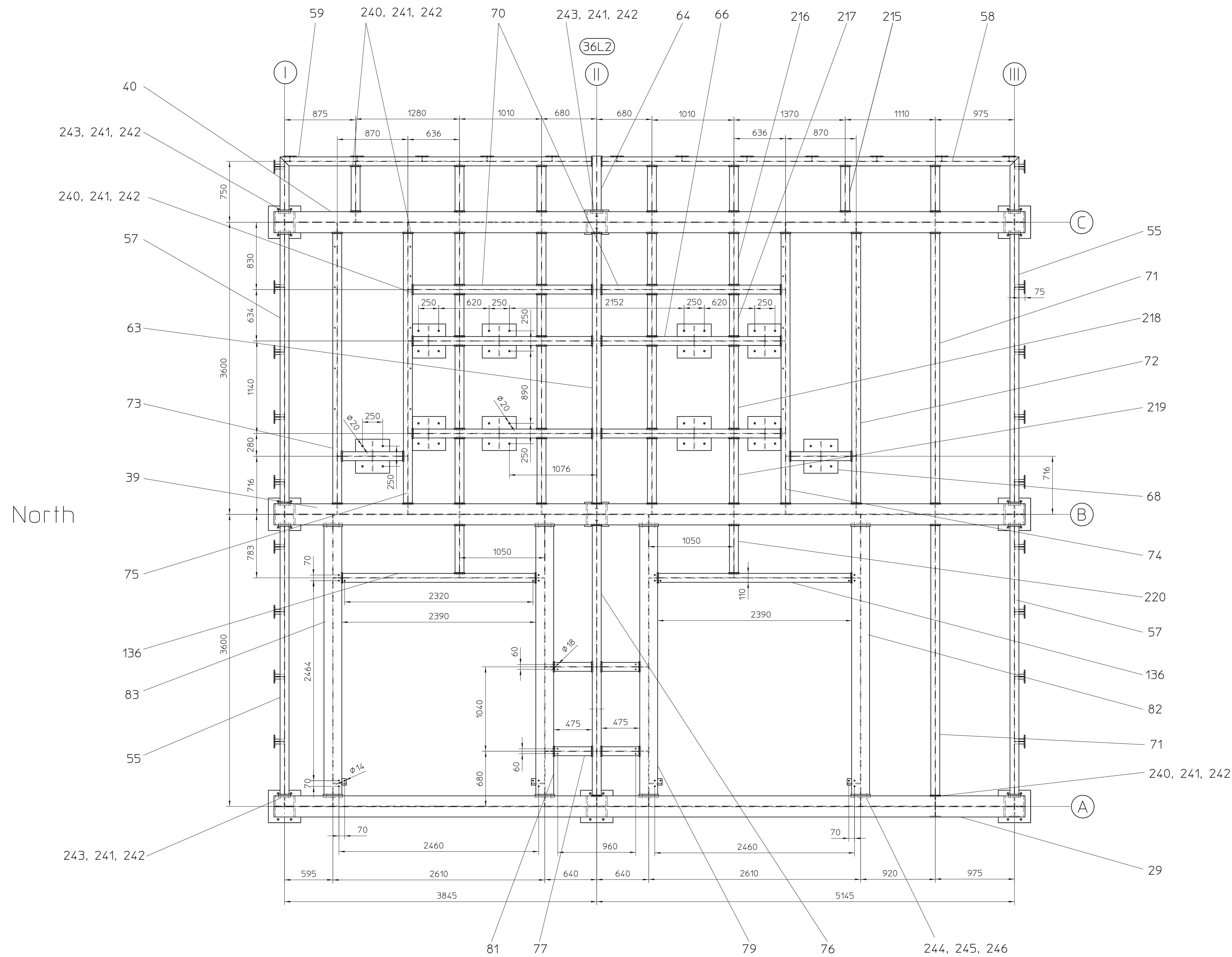
View A (without wind bracings)
