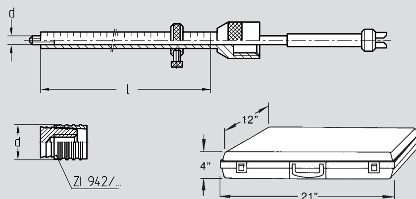
ZI 945/#2 Mounting Kit
