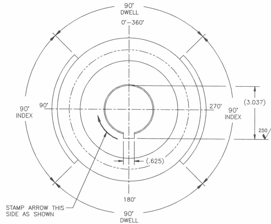
R.H. CAM TRACK DIAGRAM (REF ONLY)
