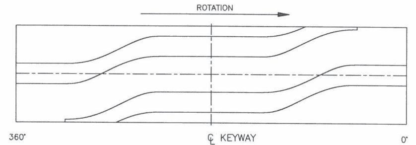
R.H. CAM TRACK DIAGRAM (REF ONLY)
