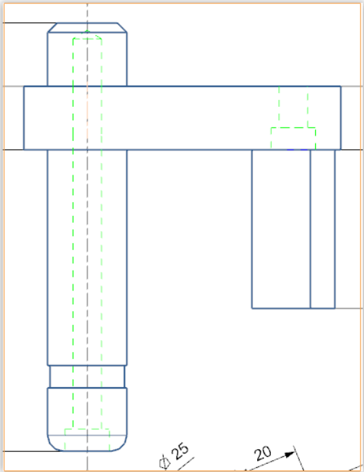
Showing specific Hidden lines
